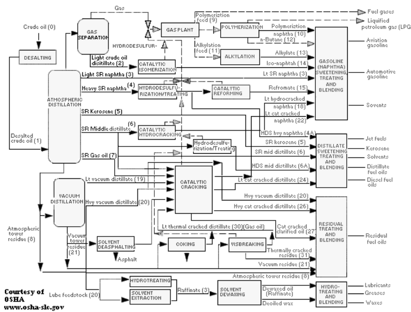
The various stages in the oil refinery process.
